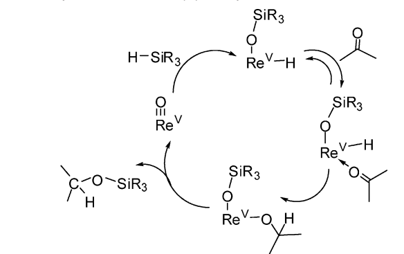
Scheme 1. Postulated Reaction Pathways for Silane Activation with Electrophilic Oxorhenium(V) Complexes
