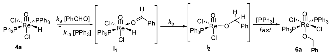
Scheme 3. Mechanism for Reaction of Et 3 SiH with the Alkoxide 6a
